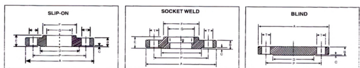
DIMENSIONS OF CLASS 150 FLANGES AS PER ANSI B 16.5
